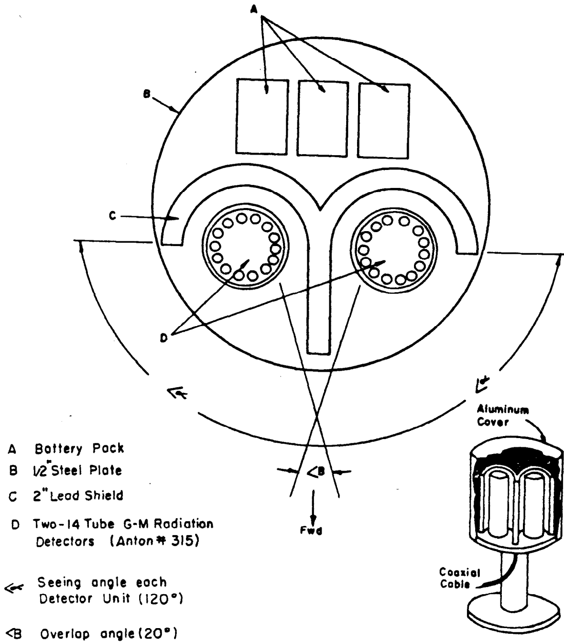
Figure 2.3 Schematic diagram of Nav-Rad unit.
